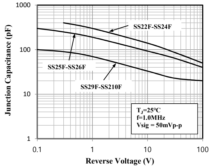
Fig.6 Typical Capacitance
